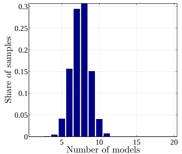
(г) K = 20, \alpha = 0.001
