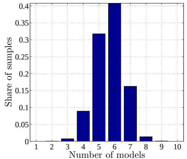
(б) K = 10, \alpha = 0.001
